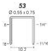
Crown 11,3mm
