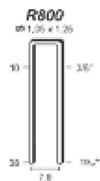
Crown 10,3mm
