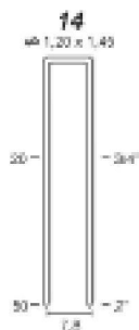
Crown 7,8mm
